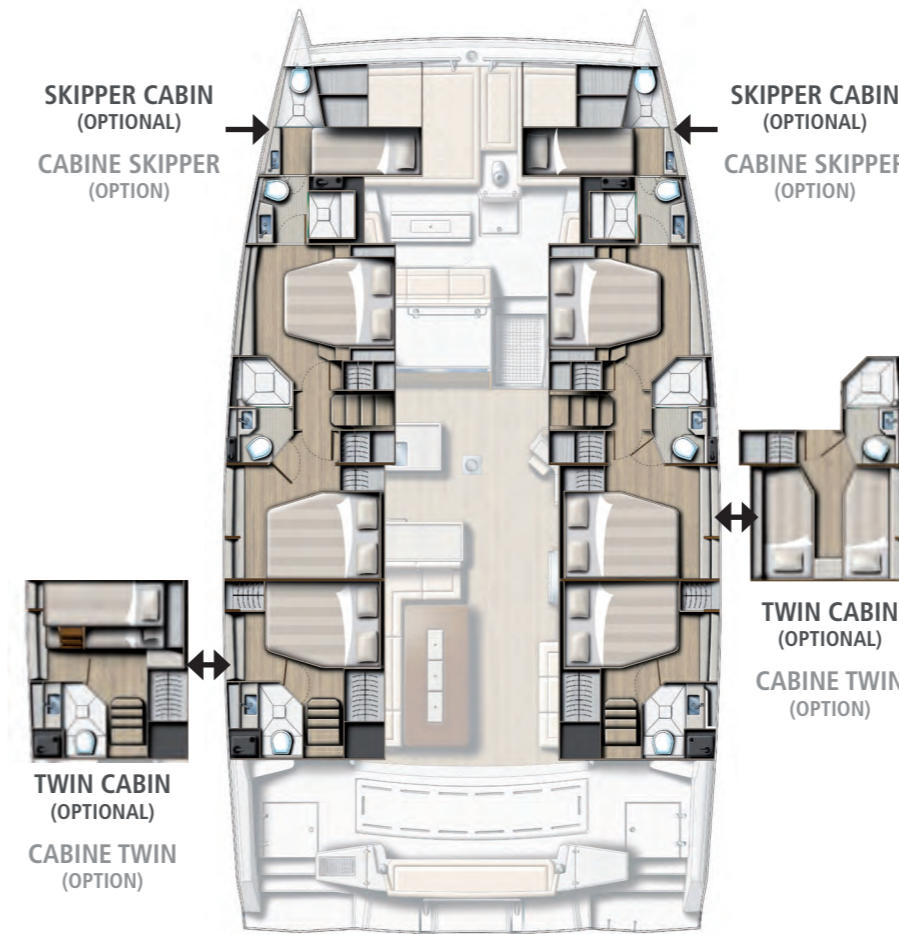
6 CABINS / 6 HEADS VERSION VERSION 6 CABINES / 6 SDB
